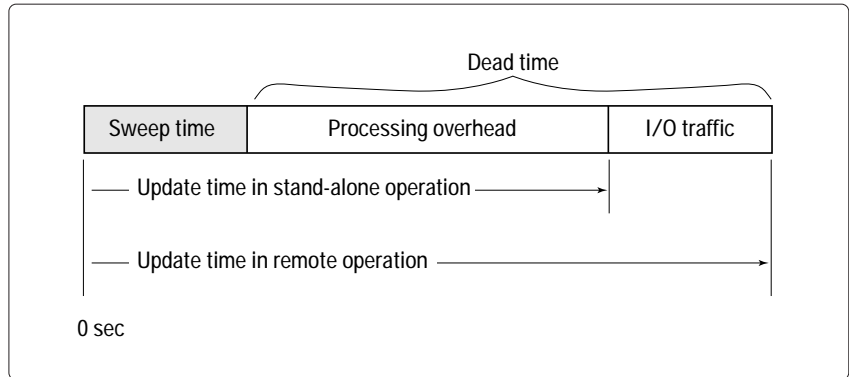
Figure 1. The components of measurement update time
