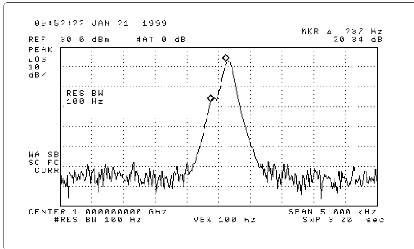
Figure 3b. 100-Hz analog RBW filter
