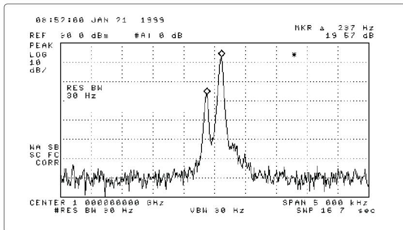
Figure 3c. 30-Hz analog RBW filter
