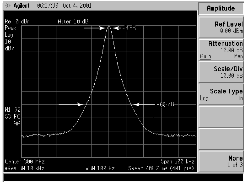
Figure 2. RBW selectivity is the ratio of the width at -60 dB to the width at -3 dB.
