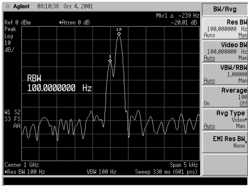
Figure 4a. 100-Hz digital RBW filter
