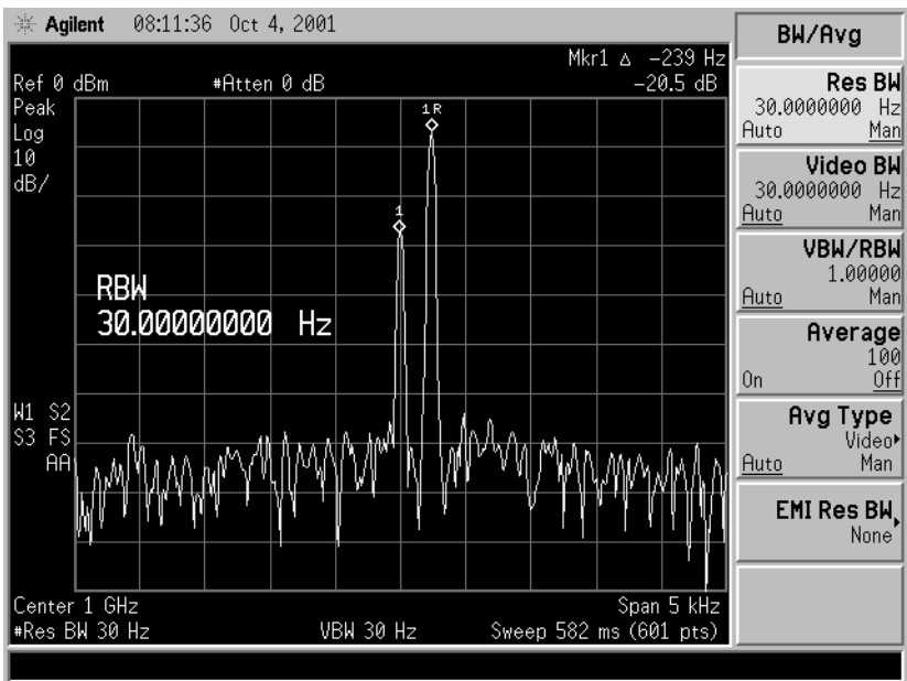
Figure 4b. 30-Hz digital RBW filter
