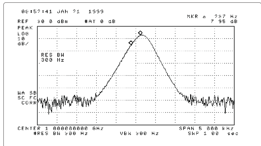
Figure 3a. 300-Hz analog RBW filter
